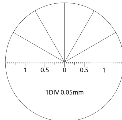
Pen Type Microscope Scale Etched into the eyepiece with graduations of 0.05mm 26800C-552 & 26800C-553
