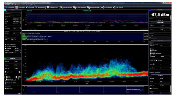
WLAN Signal
