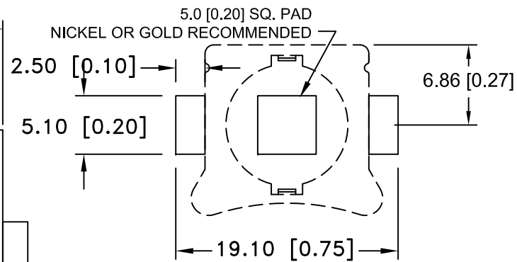
PCB LAYOUT
