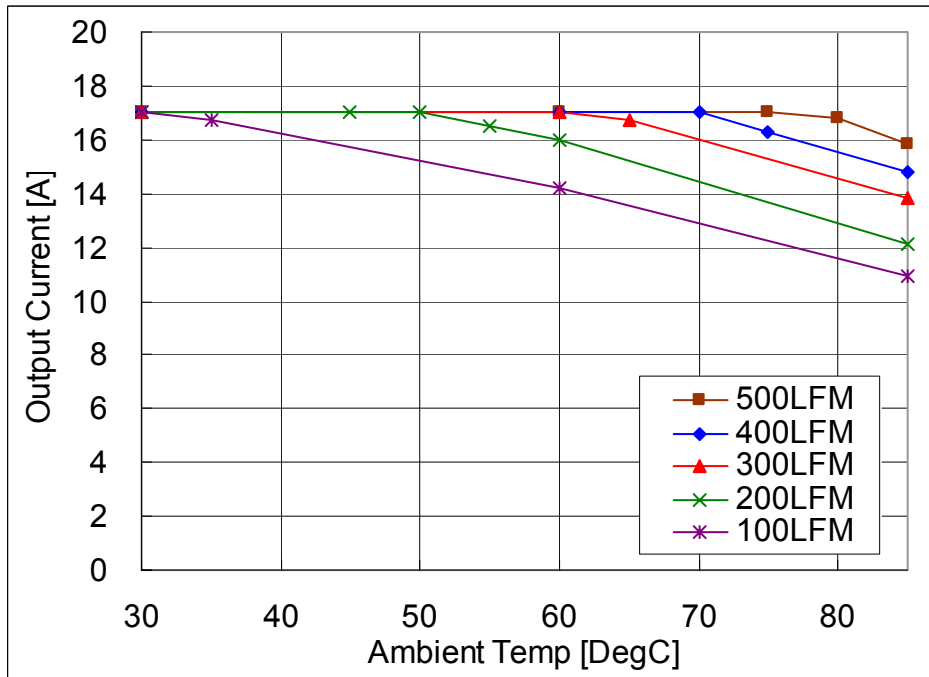
Fig.6.0V-1: Available load current vs. ambient temperature and airflow rates for Vin=48V. Maximum component temperature \leq 125^{\circ}\text{C}
