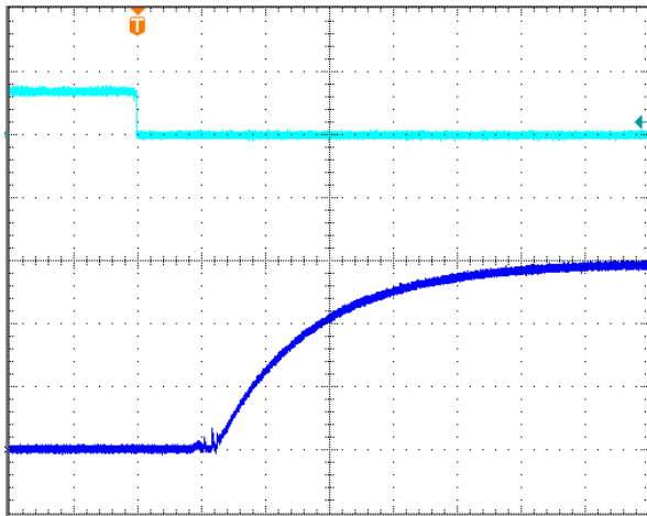
Fig.6.0V-4: Turn-on transient at full rated load current (resistive) with 10 \mu F tantalum + 1 \mu F ceramic capacitor at Vin=48V, triggered via ON/OFF pin. Top trace: ON/OFF signal (5V/div). Bottom trace: output voltage (2V/div). Time scale: 4ms/div
