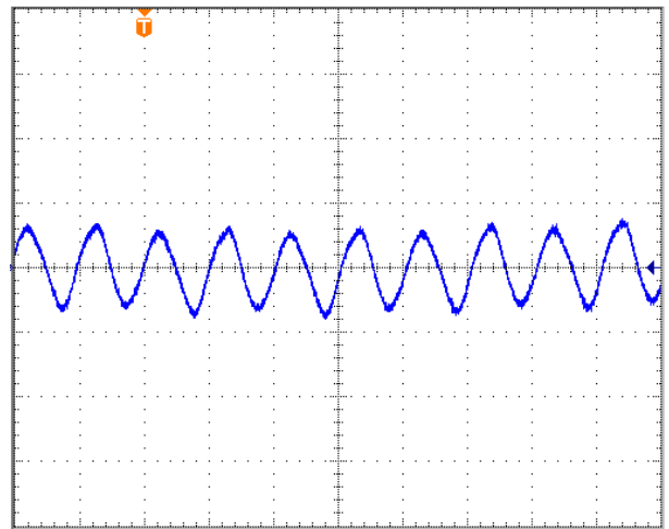
Fig.6.0V-7: Output voltage ripple (50mV/div) at full rated load current into a resistive load with Co=10 \mu F tantalum + 1 \mu F ceramic and Vin=48V. Time scale: 2 \mu s/div
