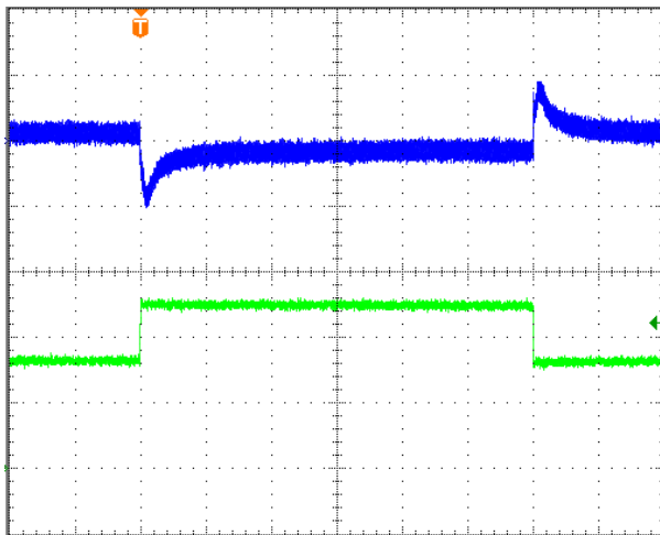
Fig.6.0V-6: Output voltage response to load current step-change (8.5A \Rightarrow 12.75A) at Vin=48V. Top trace: Output voltage (100mV/div). Bottom trace: load current (5A/div). Current slew rate: 5A/ \mu s. Co=470 \mu F os-con + 10 \mu F tantalum + 1 \mu F ceramic. Time scale: 200 \mu s/div
