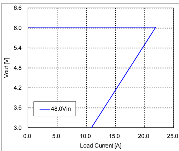
Fig.6.0V-11: Output voltage vs. load current showing current limit point and converter shutdown point. ( V_{in} = 48V )
