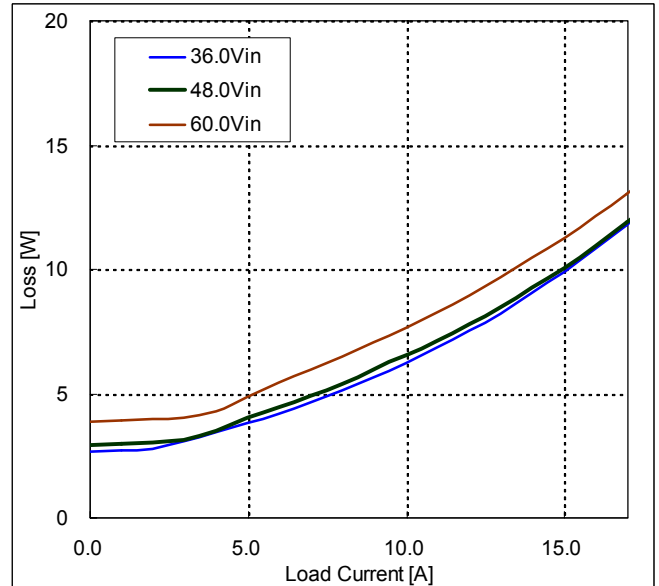
Fig.6.0V-3: Power Loss vs. load current and input voltage for converter mounted horizontally with airflow from pin 3 to pin 1 at a rate of 300LFM (1.5m/s) and Ta=25°C.
