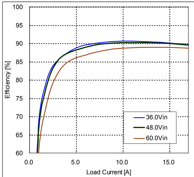
Fig.6.0V-2: Efficiency vs. load current and input voltage for converter mounted horizontally with airflow from pin 3 to pin 1 at a rate of 300LFM (1.5m/s) and Ta=25°C.
