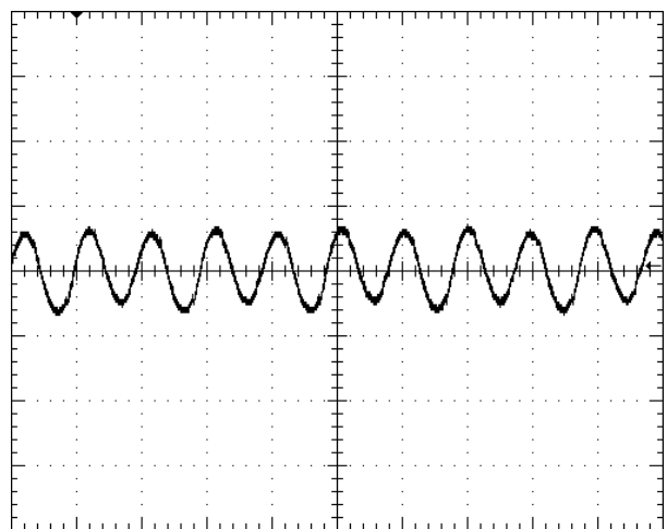
Fig.6.0V-10: Input reflected ripple current, I_c (200mA/div), measured through 10 \mu H at the source at full rated load current and V_{in}=48V . Time scale: 2 \mu s/div.
