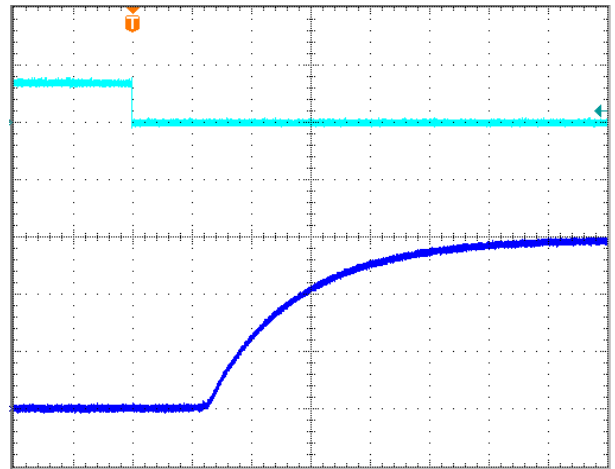
Fig.6.0V-5: Turn-on transient at full rated load current (resistive) plus 10,000 \mu F at Vin=48V, triggered via ON/OFF pin. Top trace: ON/OFF signal (5V/div). Bottom trace: output voltage (2V/div). Time scale: 4ms/div
