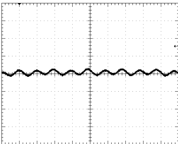
Fig.6.0V-9: Input reflected ripple current, I_s (10mA/div), measured through 10 \mu H at the source at full rated load current and V_{in}=48V . Time scale: 2 \mu s/div.
