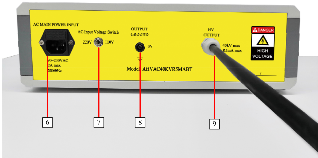
Figure 3. Front Panel
