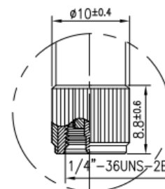
SMA(M) Connector (New)
