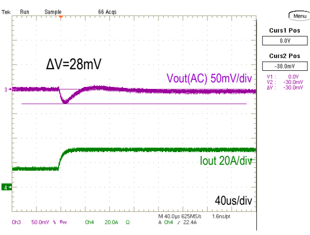
Step Load Transient Response (Vin=12.0V, Vout=0.7V, Cload=760uF, Iout=15A to 30A, 1.0A/us) Trace 3=Vout, 50mV/div, Trace 4=Iout, 20A/div.
