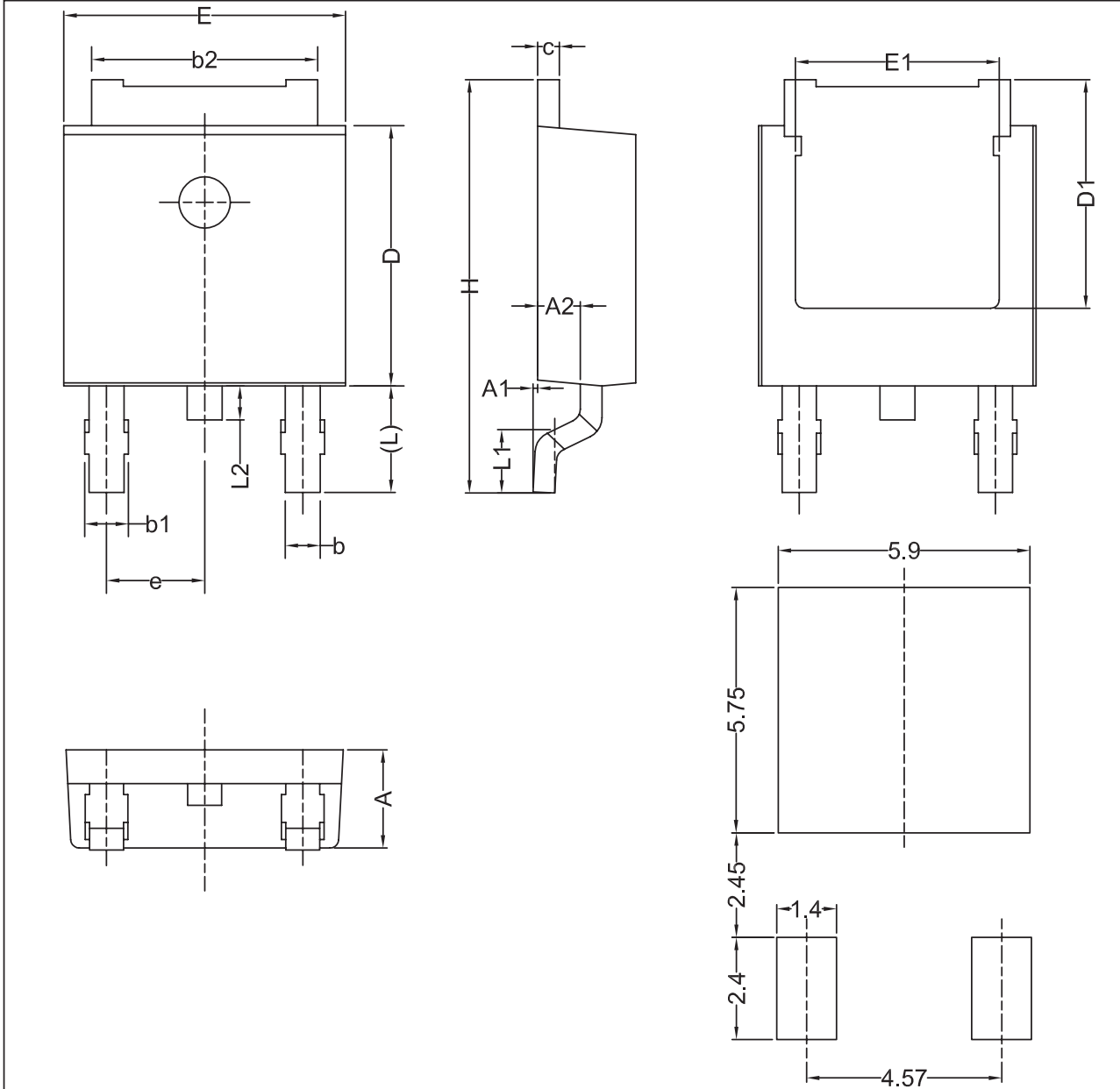
Recommended Footprint
