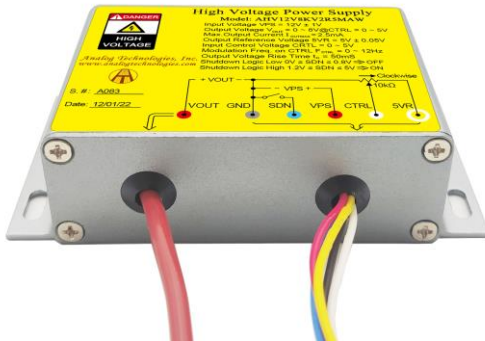
Figure 1.2. Side View
