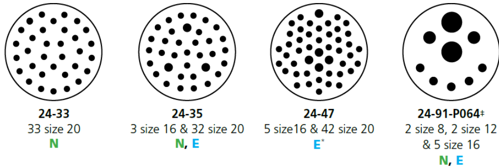
Figure 3 Pin Arrangements
