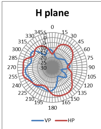
Radiation pattern, 1590 MHz
