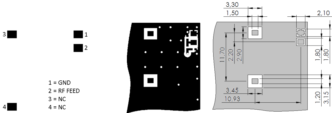
Pin configuration
