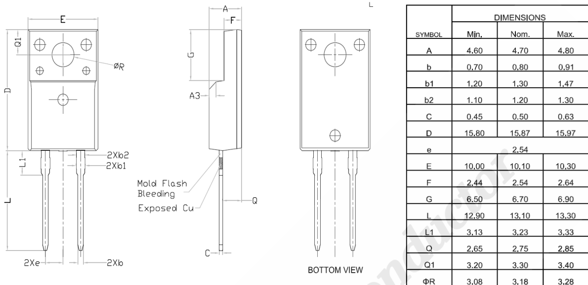
Drawing and dimensions
