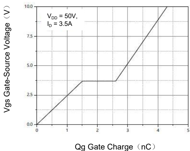
Figure 4. Gate Charge
