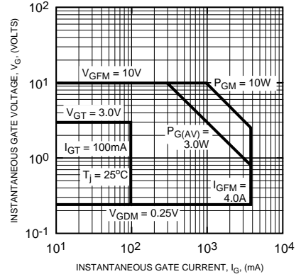
TRIGGERING CHARACTERISTICS
