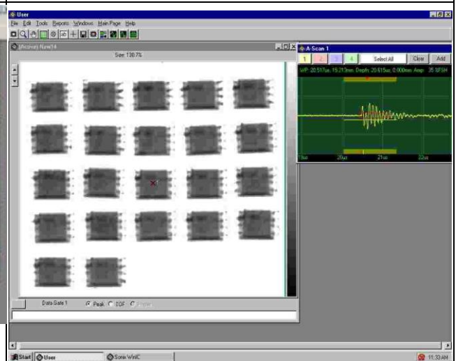
a2. Lot: 3B777600A5-1: Through Scan View
