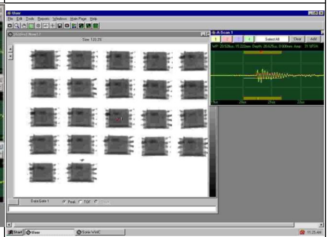
b2. Lot: 3B777600A5-2: Through Scan View
