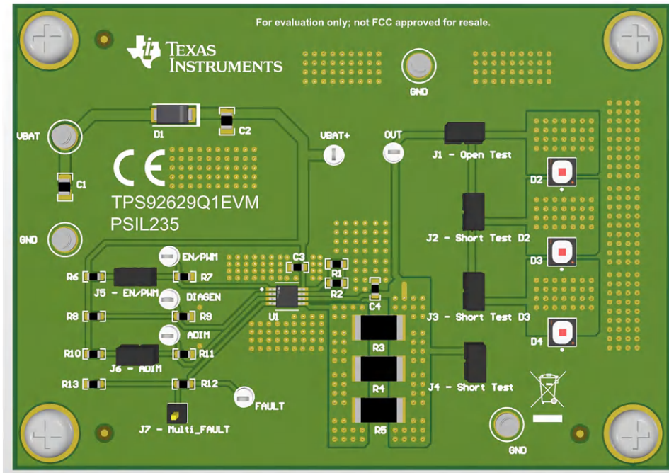
Figure 2-1. TPS92629Q1EVM Board
