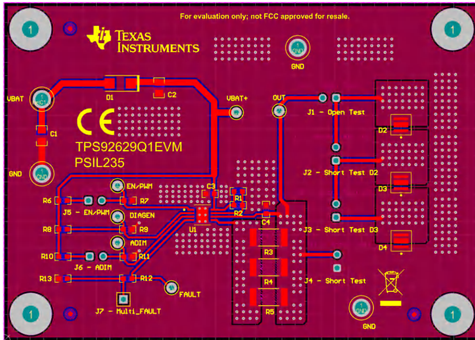
Figure 4-2. Layout
