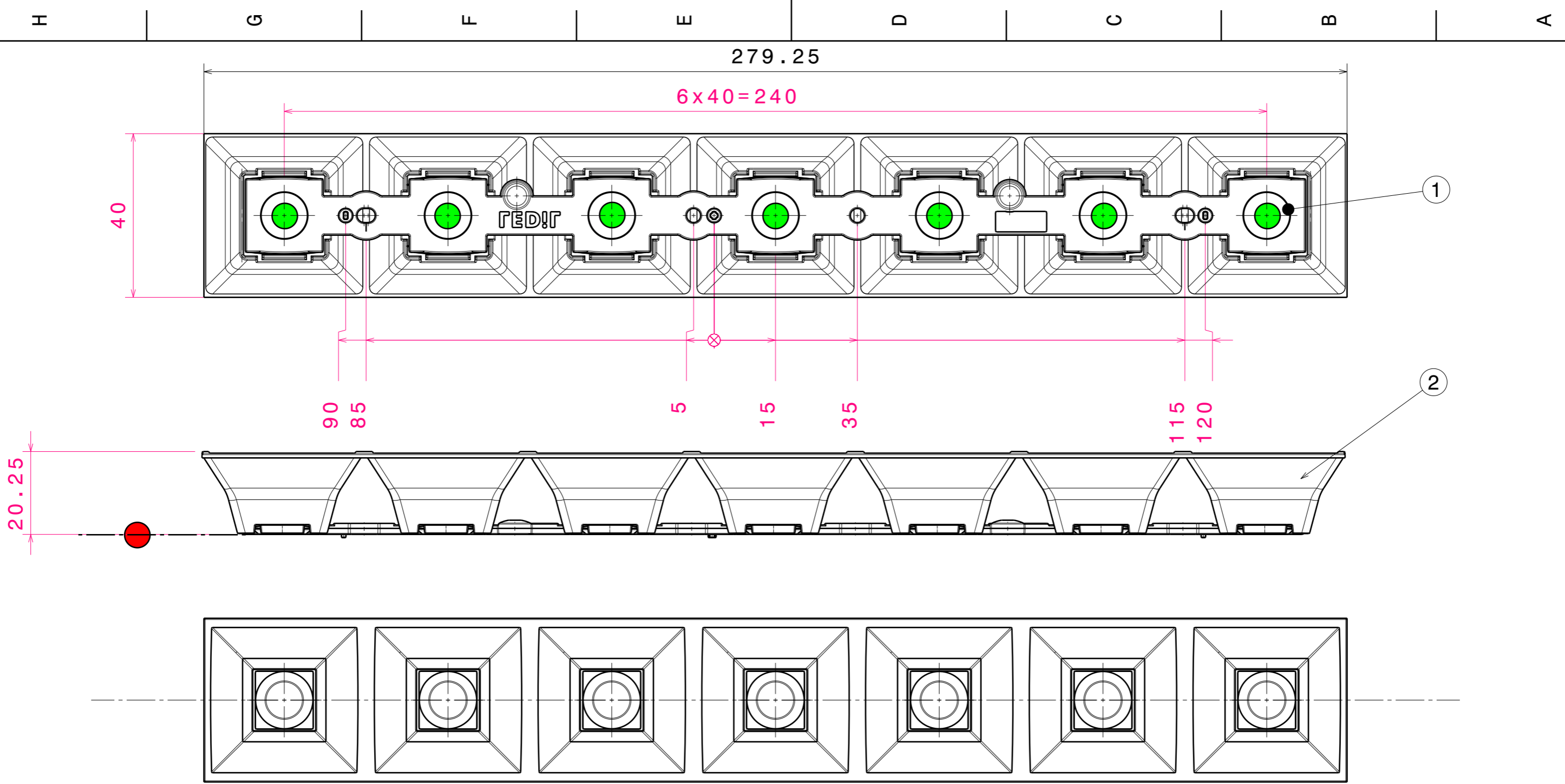
CN17367_DAISY-7X1-W2-D COMPONENTS
