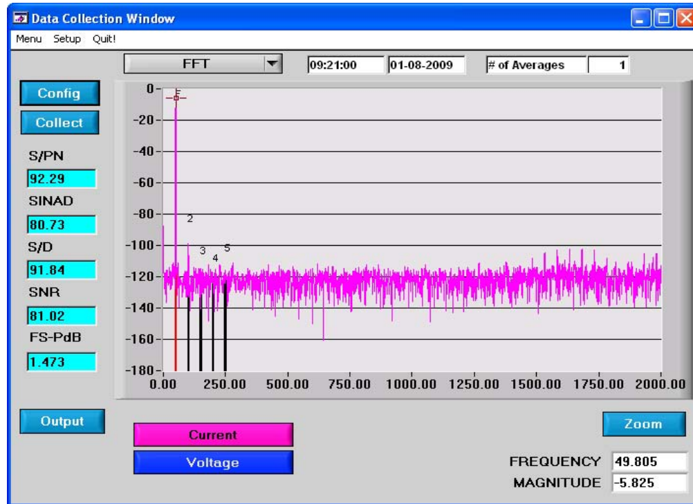
Figure 15. FFT Analysis
