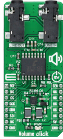
Volume Click
