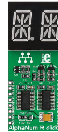
AlphaNum R Click With a dual character red LED 14-segment display and two TLC5926 16-bit shift registers. MSRP - $15 00 MIKROE-1864
