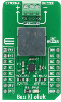
BUZZ 3 Click
