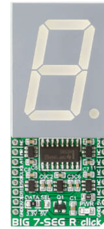
BIG 7-SEG R Click With SC10-21SR-WA seven-segment display and parallel-OUT shift register 74HC595. MSRP - $19 00 MIKROE-2269
