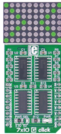
7x10 G Click With a matrix of 70 green LEDs driven by a pair of 8-bit serial-in, parallel-out shift registers. MSRP - $15 00 MIKROE-2705
