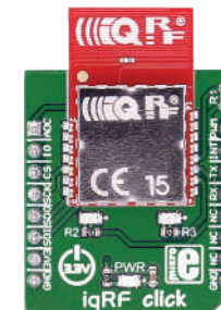
iQRF Click With DCTR-76DA RF transceiver, operating in the 868/916 MHz frequency.
