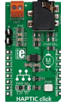
HAPTIC Click
