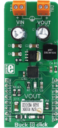
Buck 8 Click Uses the MAX17536, a high-efficiency, synchronous step-down DC-DC converter.
