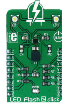
LED Flash 2 Click It is a powerful flash/torch Click, featuring the MIC2870 from Microchip. MSRP - $19 00 MIKROE-2830
