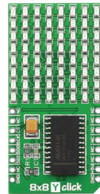
8x8 Y Click It features MAX7219 8-digit LED display driver module as well as 64 YELLOW LEDs. MSRP - $15 00 MIKROE-1294
