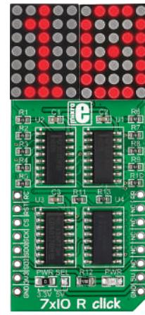
7x10 R Click With a matrix of 70 red LEDs driven by a pair of 8-bit serial-in, parallel-out shift registers. MSRP - $15 00 MIKROE-1993
