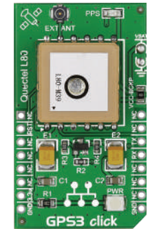
GPS3 Click With Quectel's L80, high-sensitivity GPS module with a patch antenna.
