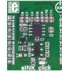
eINK Click With an adapter for connecting eINK displays, with a 24pin ribbon cable. MSRP - $59 00 MIKROE-2659
