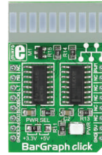
BarGraph Click With 10-segment JSB-R102510Z light bar display and two 74HC595 8-bit shift registers. MSRP - $12 00 MIKROE-1423
