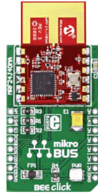
BEE Click Microchip's MRF24J-40MA 2.4 GHz IEEE 802.15.4 radio transceiver module.
