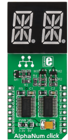
AlphaNum G Click With a dual character green LED 14-segment display and two TLC5926 16-bit shift registers. MSRP - $15 00 MIKROE-1851
