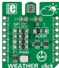
Weather Click With BME280 integrated environmental unit. Detects humidity, pressure, and temperature. MSRP - $22 00 MIKROE-1978
