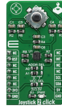
Joystick 2 Click
