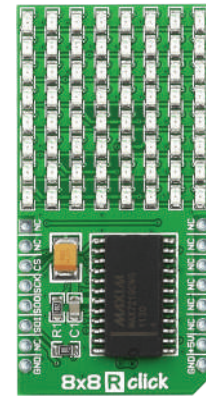
8x8 R Click It features MAX7219 8-digit LED display driver module as well as 64 RED LEDs. MSRP - $15 00 MIKROE-1295
