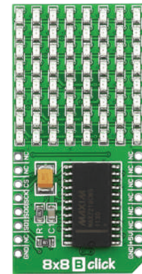
8x8 B Click It features MAX7219 8-digit LED display driver module as well as 64 BLUE LEDs. MSRP - $18 00 MIKROE-1307
