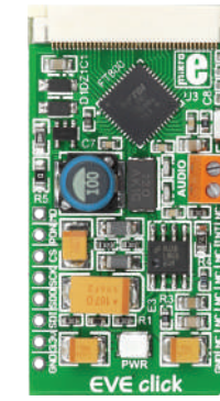
EVE Click Brings visually stunning graphics even to 8-bit MCUs, with FT800Q graphics controller. MSRP - $39 00 MIKROE-1430
