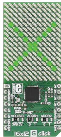
16x12 G Click Carries a 16x12 LED display and the IS-31FL3733 matrix driver with 1/12 cycle rate. MSRP - $30 00 MIKROE-2758
