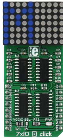
7x10 B Click With a matrix of 70 blue LEDs driven by a pair of 8-bit serial-in, parallel-out shift registers. MSRP - $15 00 MIKROE-2789
