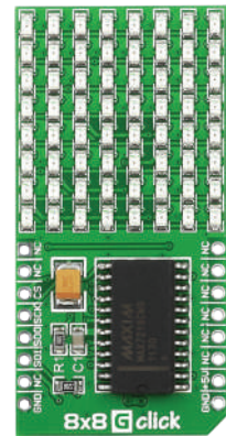
8x8 G Click It features MAX7219 8-digit LED display driver module as well as 64 GREEN LEDs. MSRP - $15 00 MIKROE-1306
