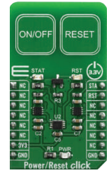
Power/Reset Click
