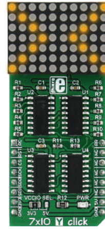
7x10 Y Click With a matrix of 70 yellow LEDs driven by a pair of 8-bit serial-in, parallel-out shift registers. MSRP - $15 00 MIKROE-2790
