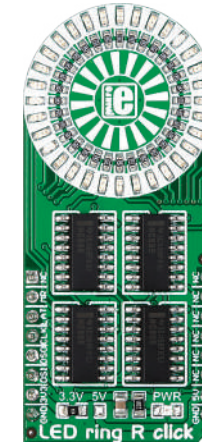
Led ring R Click With a ring of 32 red LEDs driven by four 74HC595 serial-in, parallel-out shift registers. MSRP - $16 00 MIKROE-2153
