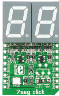
7seg Click 2-digit seven-seg display. With two 74HC595 8-bit serial-in, parallel-out shift registers. MSRP - $10 00 MIKROE-1201
