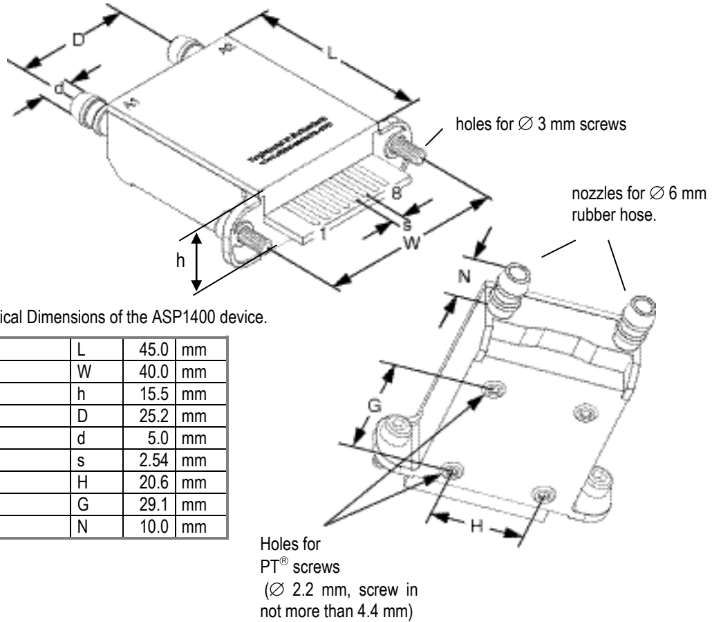
Figure 12: Physical dimensions and mounting information of the ASP1400.
