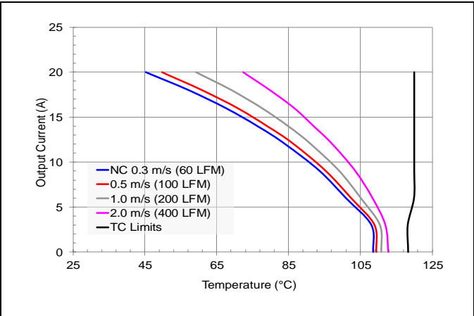
V_o = 12\text{ V} , V_{in} = 24\text{ V} preliminary maximum output current vs. ambient temperature at nominal input voltage for natural convection (60lfm) to 400lfm with airflow from pin 8 to pin 4.
