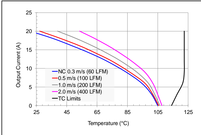
V_o = 5\text{ V} , V_{in} = 36\text{ V} preliminary maximum output current vs. ambient temperature at nominal input voltage for natural convection (60lfm) to 400lfm with airflow from pin 8 to pin 4.
