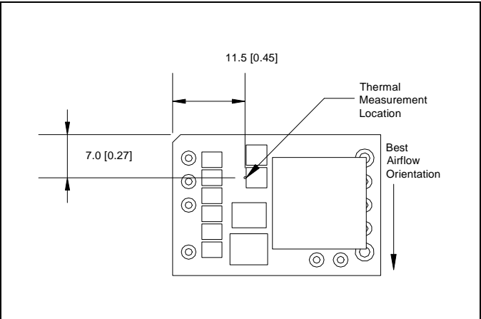
i6A4W010A033V thermal measurement location ( T_c ) – top view
