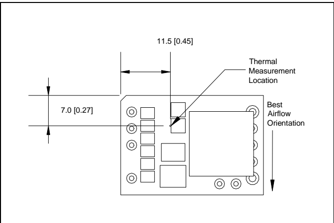
i6A4W020A033V thermal measurement location ( T_c ) – top view
