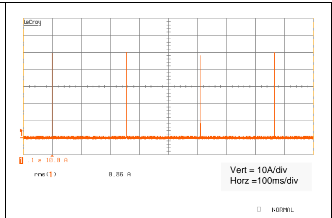
Typical Output Short Circuit Current – CH1, orange
