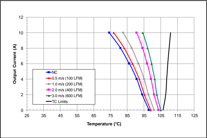
V_o = 12\text{ V} , V_{in} = 24\text{ V} preliminary maximum output current vs. ambient temperature at nominal input voltage for natural convection (60lfm) to 600lfm with airflow from pin 8 to pin 4.
