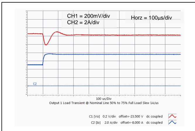
Vo = 24 V Typical output voltage transient response to load step from 50% to 75% of full load with output current slew rate of 1 A/µs (Cext = 22 µF).
