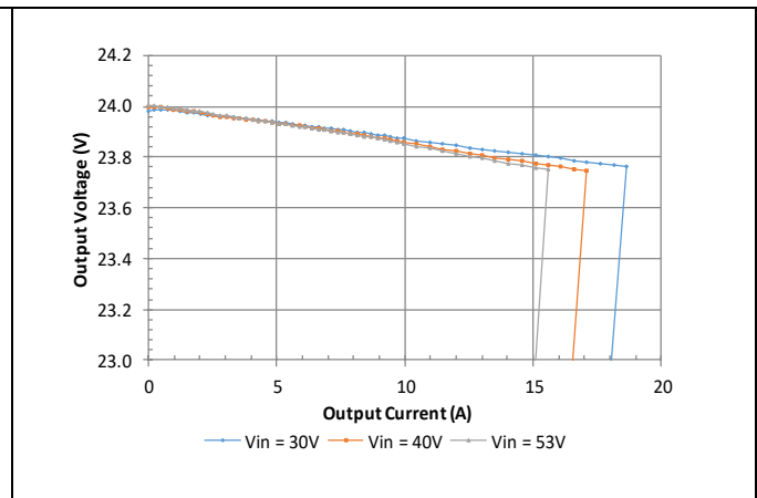
Vo = 24 V Typical Current Limit Characteristics
