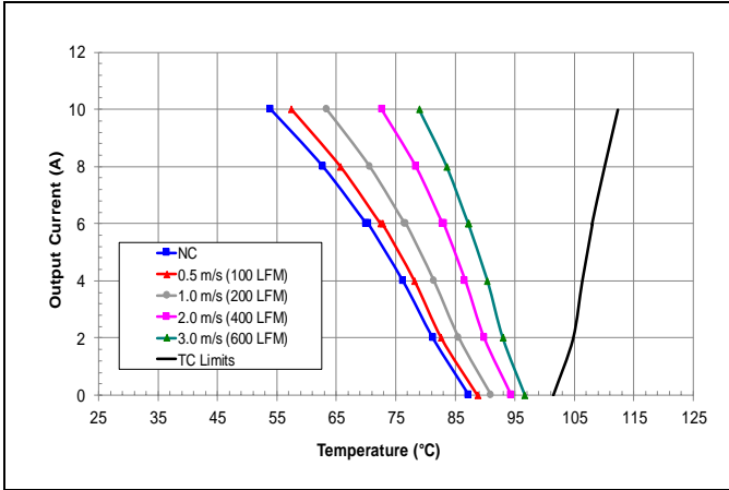
V_o = 24\text{ V} , V_{in} = 36\text{ V} preliminary maximum output current vs. ambient temperature at nominal input voltage for natural convection (60lfm) to 600lfm with airflow from pin 4 to pin 3.
