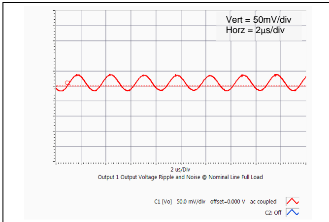
Vo = 24 V Typical Output Ripple at nominal Input voltage and full load at Ta = 25 °C.
