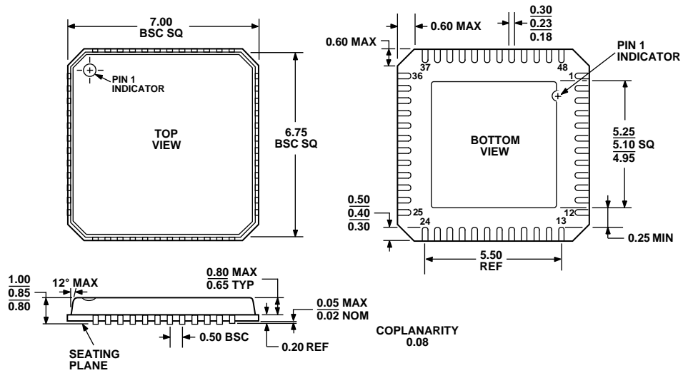
COMPLIANT TO JEDEC STANDARDS MO-220-VKKD-2 Figure 8. 48-Lead Frame Chip Scale Package [LFCSP] (CP-48)
