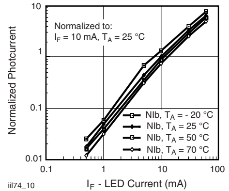
Fig. 13 - Normalized Photocurrent vs. I_F and Temperature
