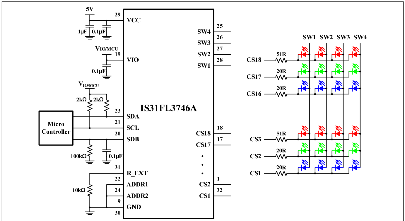
Figure 1 Typical Application Circuit: 18×4, 24 RGBs
