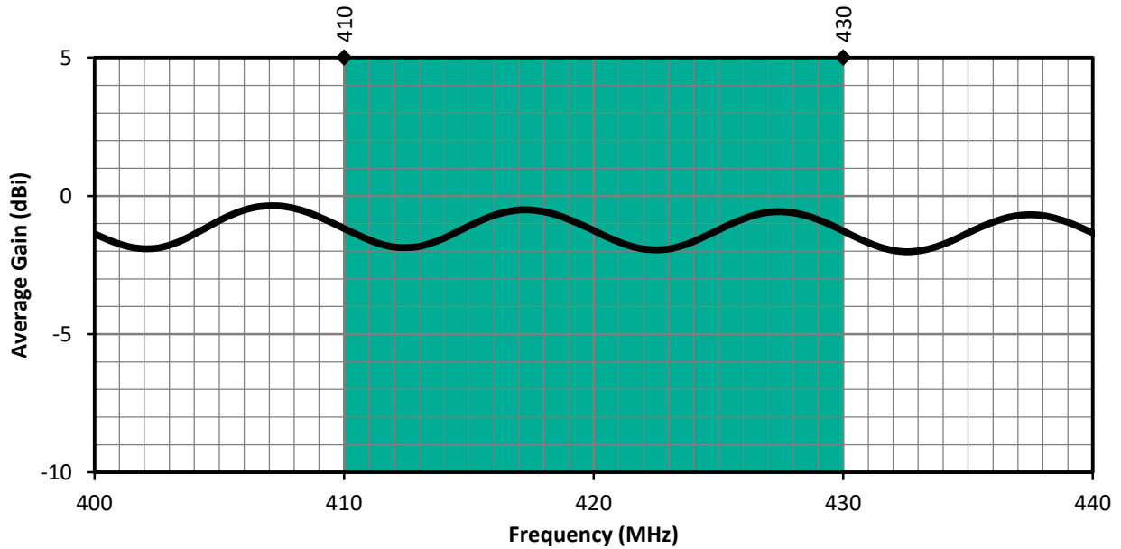
Figure 4. PW 410 MHz Antenna Average Gain with Band Highlight
