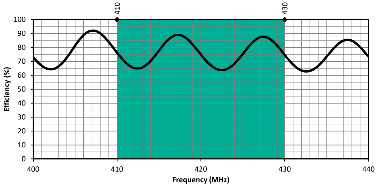
Figure 5. PW 410 MHz Antenna Radiation Efficiency with Band Highlight
