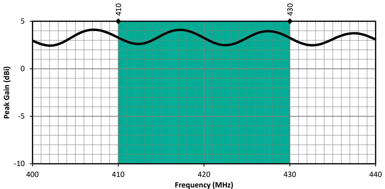
Figure 3. PW 410 MHz Antenna Peak Gain with Band Highlight
