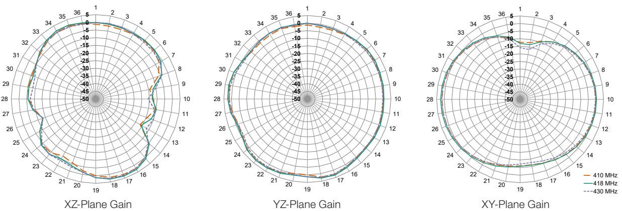
Figure 8. Radiation Patterns for PW 410 MHz Antenna
