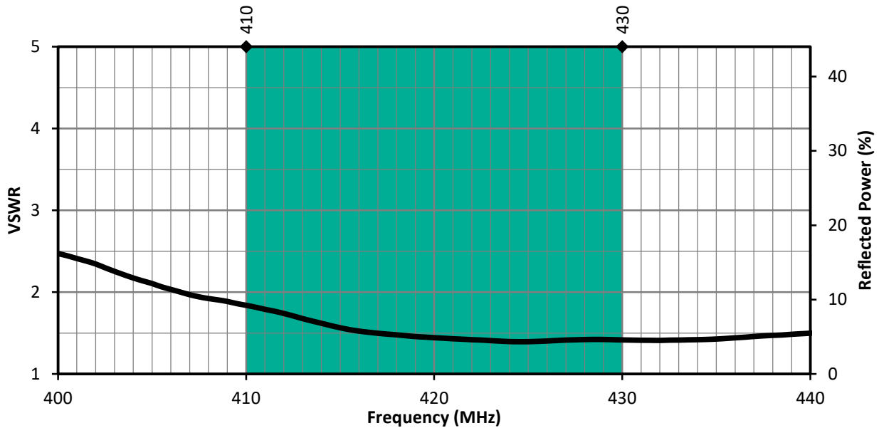
Figure 1. PW 410 MHz Antenna VSWR with Band Highlight
