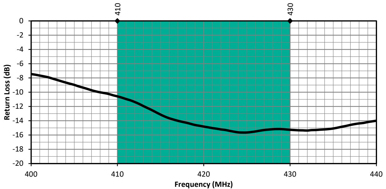
Figure 2. PW 410 MHz Antenna Return Loss with Band Highlight
