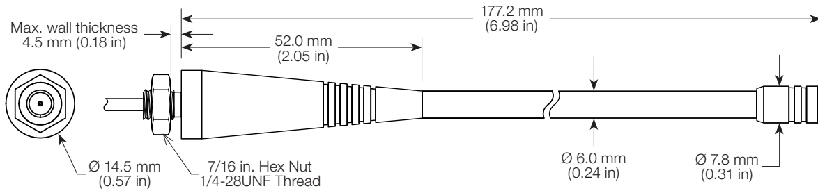
Figure 6. PW 410 MHz Antenna Dimensions
