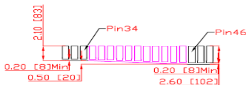
Detail C
