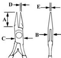
2847D Needle Nose Plier Serrated Jaw
