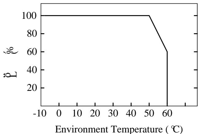
Figure 26. Derating Curve
