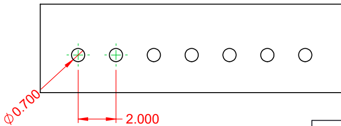
SUGGESTED PCB LAYOUT
