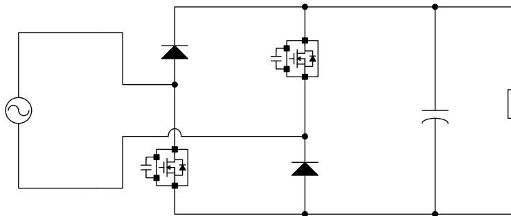
Figure 24. Application Circuit 6
