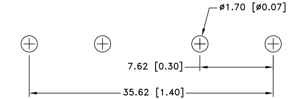
MOUNTING DETAIL
