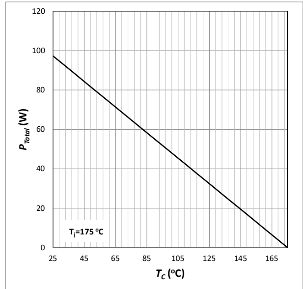
Fig. 4 Power Derating
