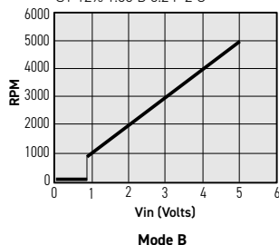
VPWM-pos-slope 2008/7/16 RPM: 882 to 5000 Vs: 1.8 to 10 Volts MODE: TYPE- B change @: 1.78 V VPWM 1.8 10 18 100 B 500 ST 12% 1.65 D 0.2 F 2 C
