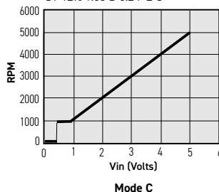
VPWM-pos-slope 2008/7/16 RPM: 882 to 5000 Vs: 1.8 to 10 Volts VPWM 1.8 10 18 100 C 500 MODE: TYPE- C change @: 0.8 V ST 12% 1.65 D 0.2 F 2 C
