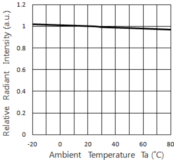
Relative Radiant Intensity & Ambient Temperature
