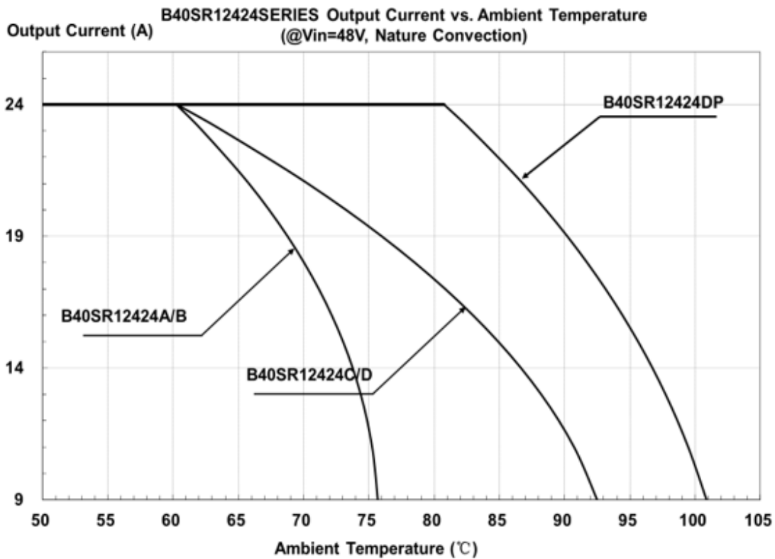
Figure 23: Output Current vs. Ambient temperature @ Vin=48V
