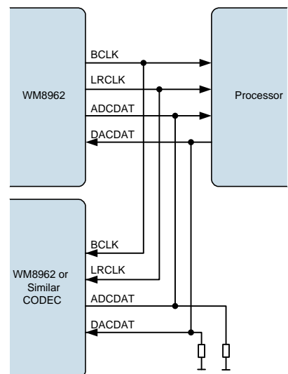
Figure 40 TDM with WM8962 as Master
