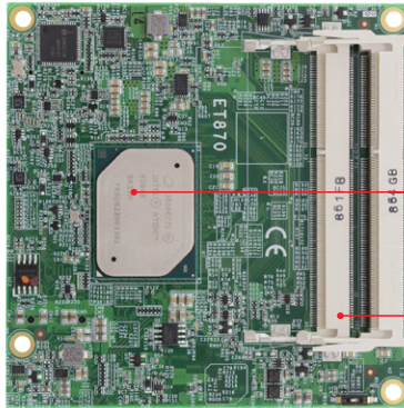
Intel® Atom® x7x5 CPU DDR3L SO-DIMM Sockets
