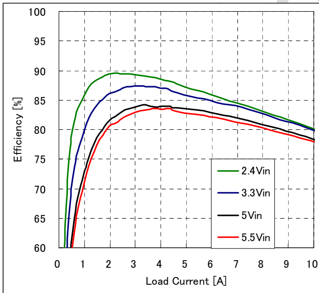
Fig-0.7525V-2: Efficiency vs. load current and input voltage for Vout=0.7525V. Airflow rate=200 LFM (1.0m/s) and Ta=25°C.
