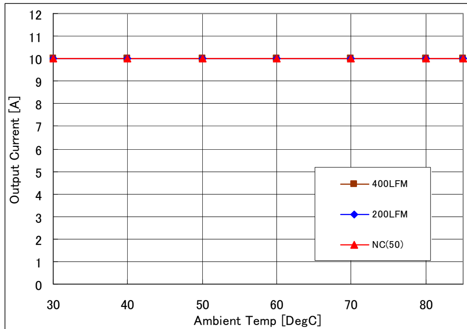
Fig-0.7525V-1: Available load current vs. ambient temperature and airflow rates for Vout=0.7525V with Vin=5.0V. Maximum component temperature ≤ 120°C
