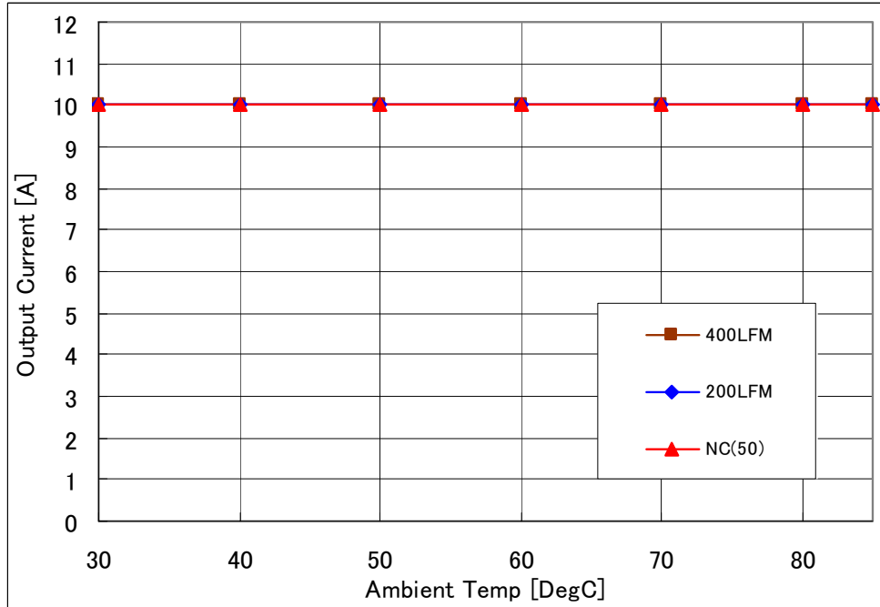
Fig-1.8V-1: Available load current vs. ambient temperature and airflow rates for Vout=1.8V with Vin=5.0V. Maximum component temperature ≤ 120°C
