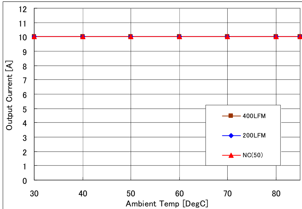
Fig-2.5V-1: Available load current vs. ambient temperature and airflow rates for V_{out}=2.5V with V_{in}=5.0V . Maximum component temperature \leq 120^{\circ}C
