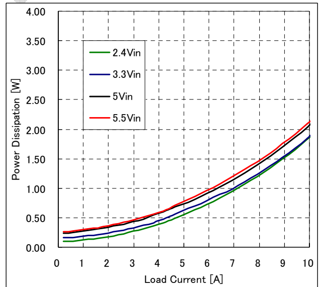
Fig-0.7525V-3: Power dissipation vs. load current and input voltage for Vout=0.7525V. Airflow rate=200 LFM (1.0m/s) and Ta=25°C.
