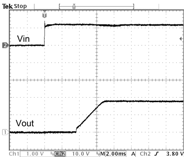
Fig.12: Turn on delay time at 12Vin, 1.8V/3A out
