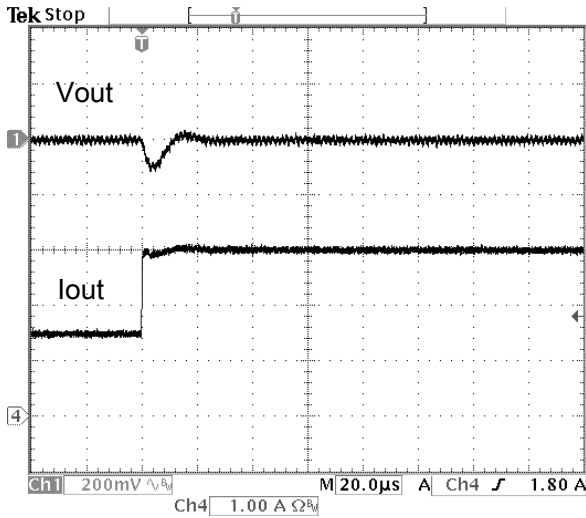
Fig.14: Output voltage response to step load change at 5A/us from 50% to 100% (12V in , 1.8V out )
