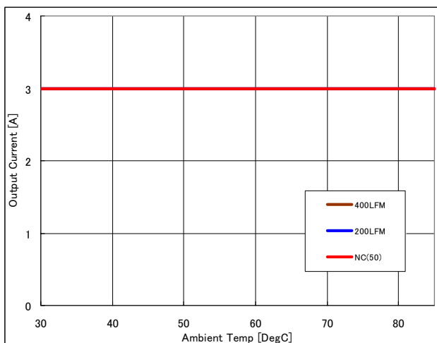
Fig.1: Output current vs. ambient temperature and air velocity at 12Vin, 1.8V to 6.6V out
