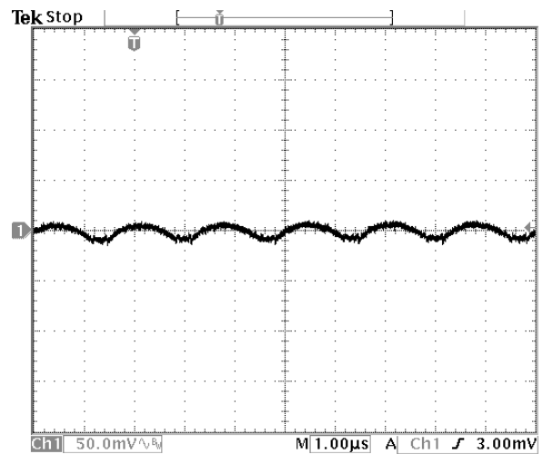
Fig.13: Output ripple and noise at 12Vin, 1.8V/3Aout
