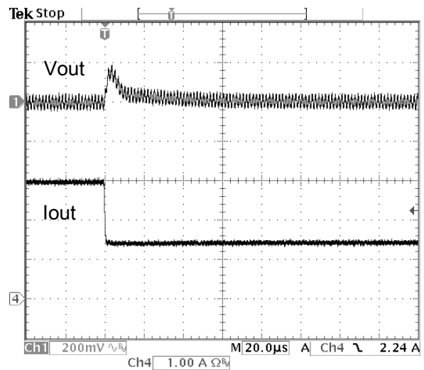
Fig.11: Output voltage response to step load change at 5A/us from 100% to 50% (12Vin, 6.6Vout)
