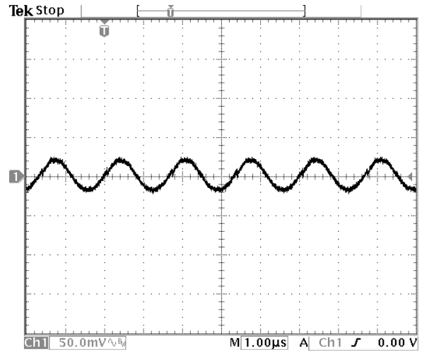
Fig.9: Output ripple and noise at 12Vin, 6.6V/3Aout
