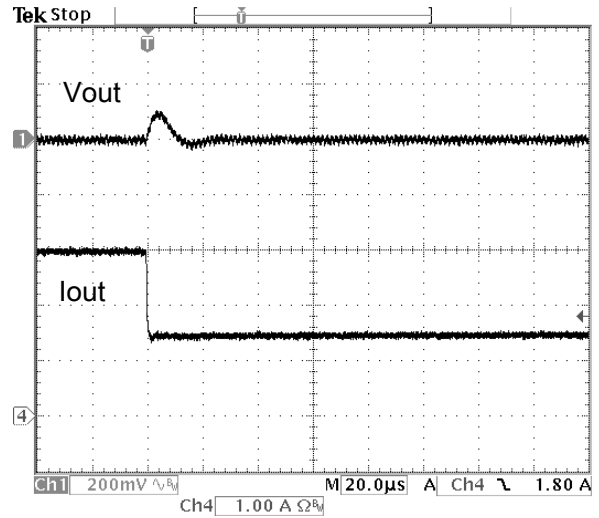
Fig.15: Output voltage response to step load change at 5A/us from 100% to 50% (12V in , 1.8V out )
