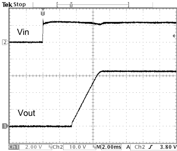
Fig.8: Turn on delay time at 12Vin, 6.6V/3A out
