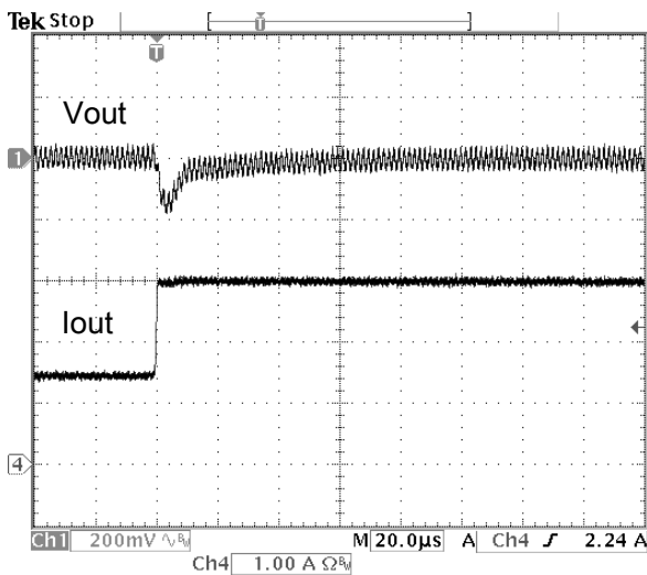
Fig.10: Output voltage response to step load change at 5A/us from 50% to 100% (12Vin, 6.6Vout)
