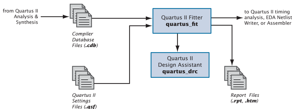
Figure 1. Place and Route Design Flow
