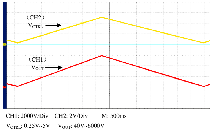
Figure 4. Triangle Wave
