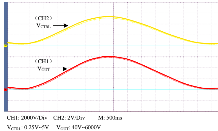
Figure 5. Sine Wave
