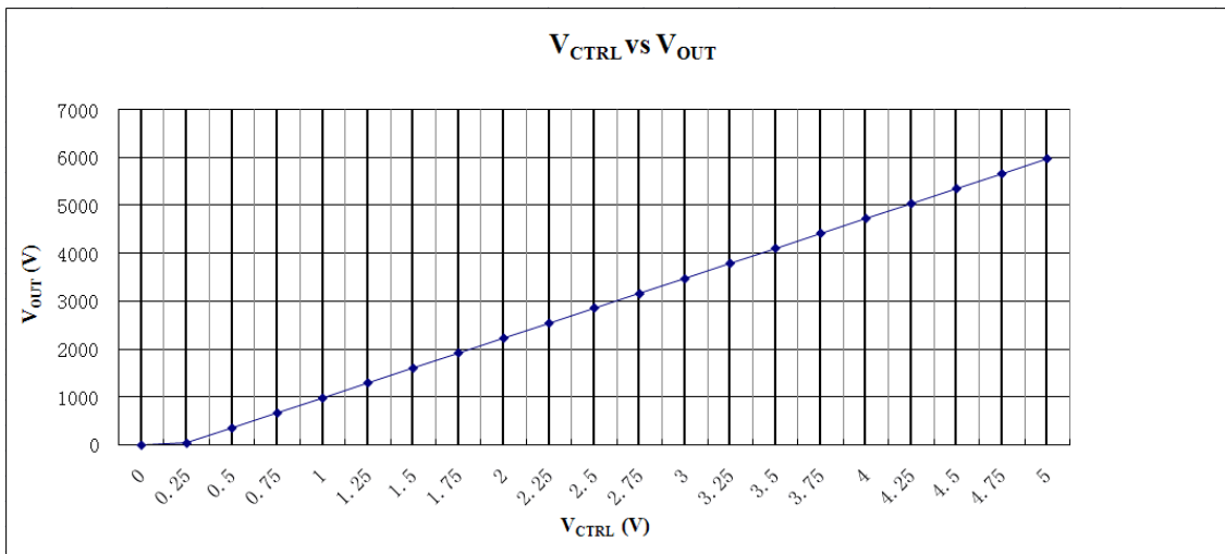
Figure 3. V_CTRL vs. V_OUT
