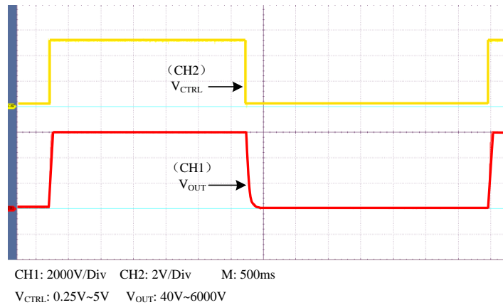
Figure 6. Square Wave
