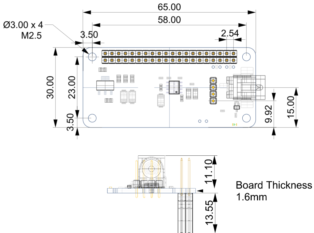
Figure 2 Mechanical Dimensions (mm)
