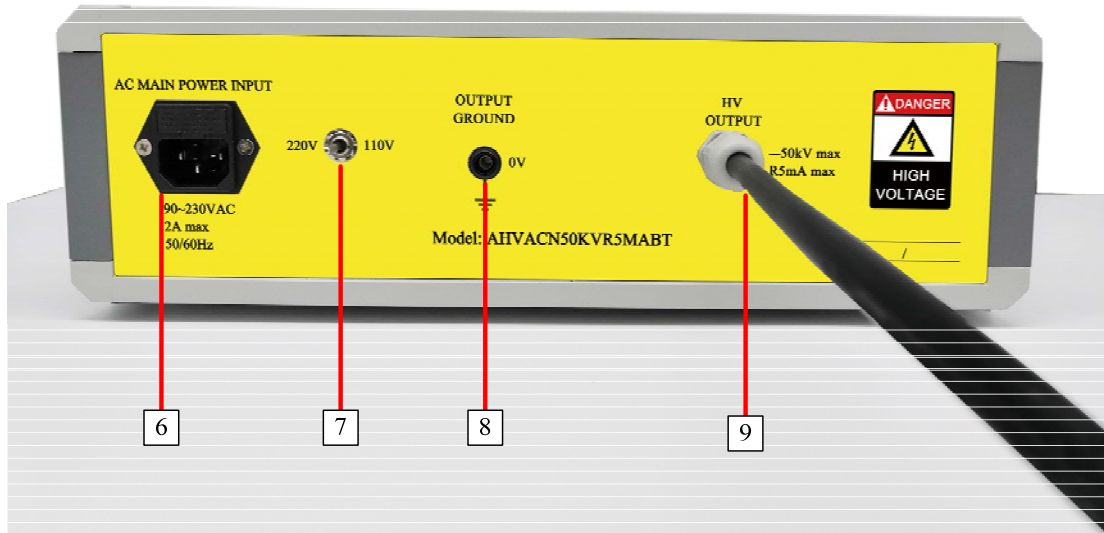
Figure 3. Back Panel
