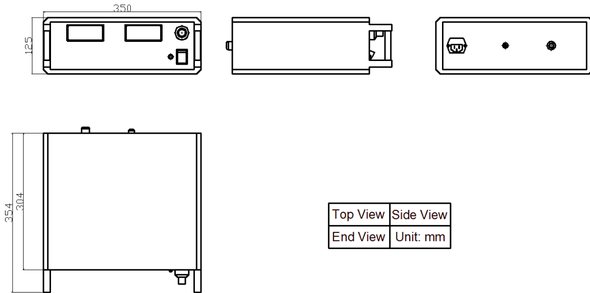
Figure 7. Dimensions for AHVACN50KVR5MABT
