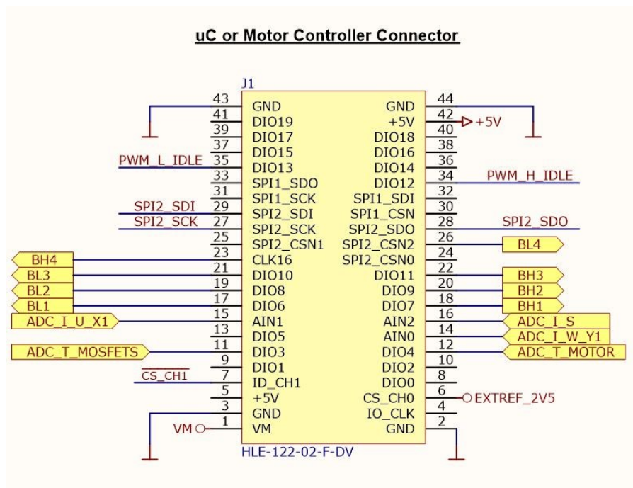
Figure 1: 44 pin Motor Controller Connector
