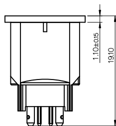
Straight Plug With Cap
